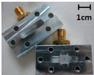
① 超伝導空洞共振器と超伝導量子ビット素子 Superconducting quantum bit inside a superconducting cavity
