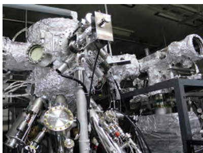
② 分子線エピタキシー結晶成長装置 Molecular beam epitaxy (MBE) for single-crystal semiconductor growth
