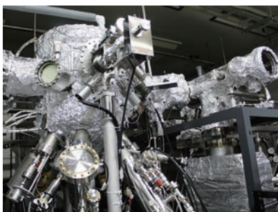
2 分子線エピタキシー結晶成長装置 Molecular beam epitaxy (MBE) for single-crystal semiconductor growth
